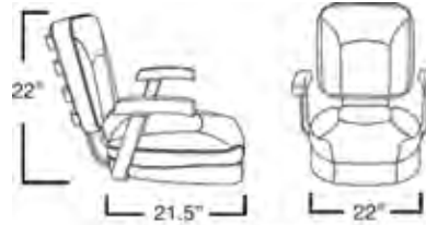
Seat Dimensions
