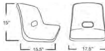
Seat Dimensions
